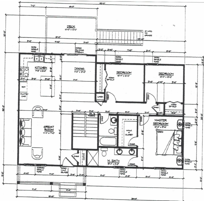
MAIN FLOOR PLAN 1/4" = 1'-0"
