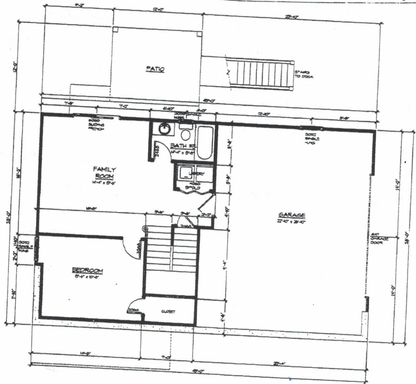
LOWER FLOOR PLAN 1/4" = 1'-0"
